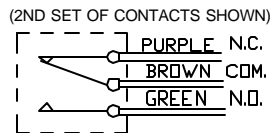
DPDT- K331/332
