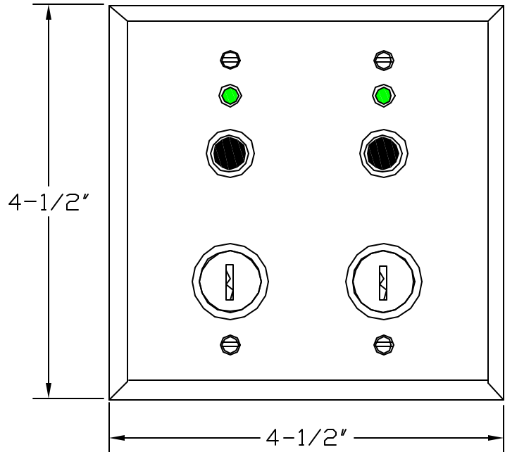
2 GANG PLATE
