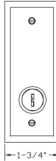
NARROW PLATE
